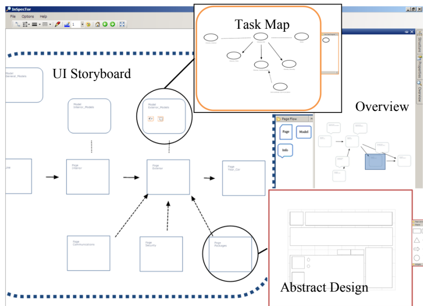
Fig. 4. UI storyboard with UI design and models (magnified areas for illustration).
