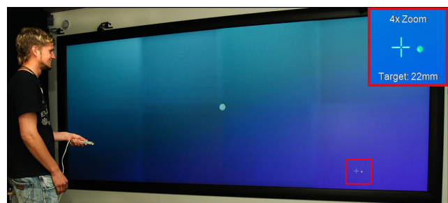
Fig. 12 Laser Pointer Interaction in front of a large high-resolution display. Squidy facilitated the integration and evaluation of precision enhancing and smoothing techniques, allowing the precise selection of targets as small as 22mm in diameter from a 3m distance [21].
