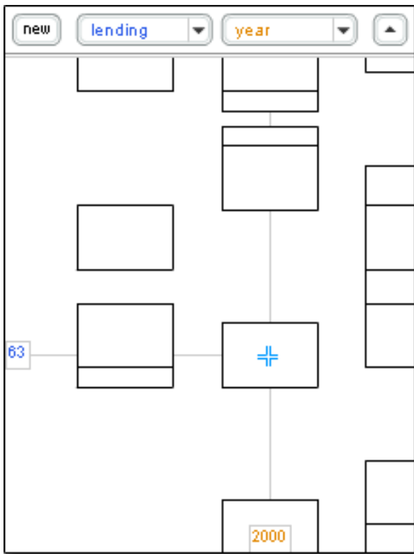
Figure 4: Geometric zoom.
