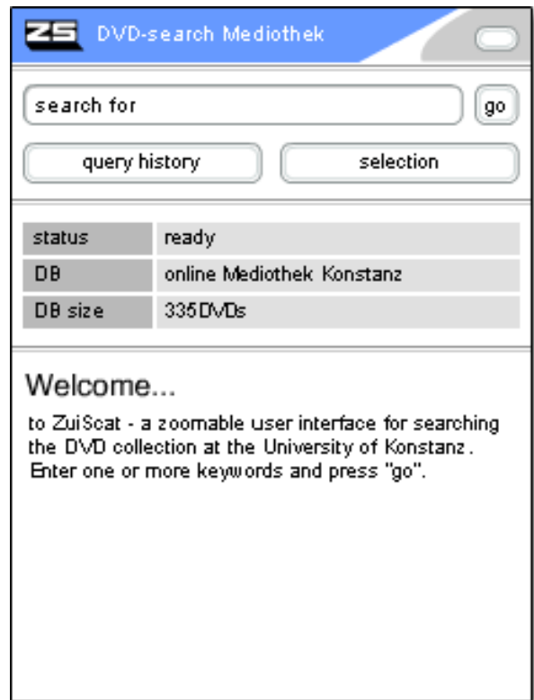
Figure 1: Start screen.
