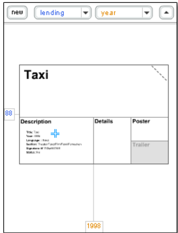
Figure 5: Semantic zoom.
